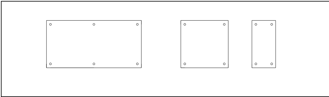
Figure 1 Fixing layouts – minimum fixing numbers (for solely mechanically fixed specification)
